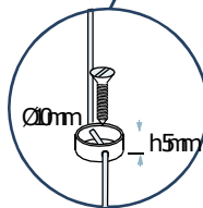
Tendicavo / Piano
